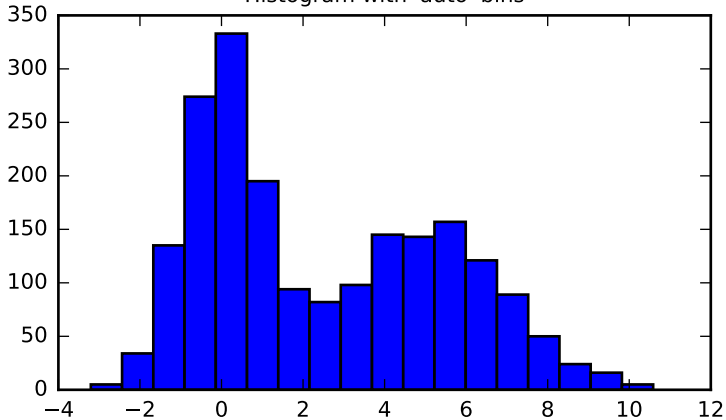
Histogram with 'auto' bins
